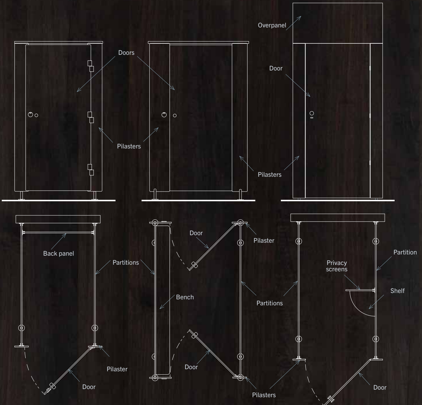
Double entry cubicle
